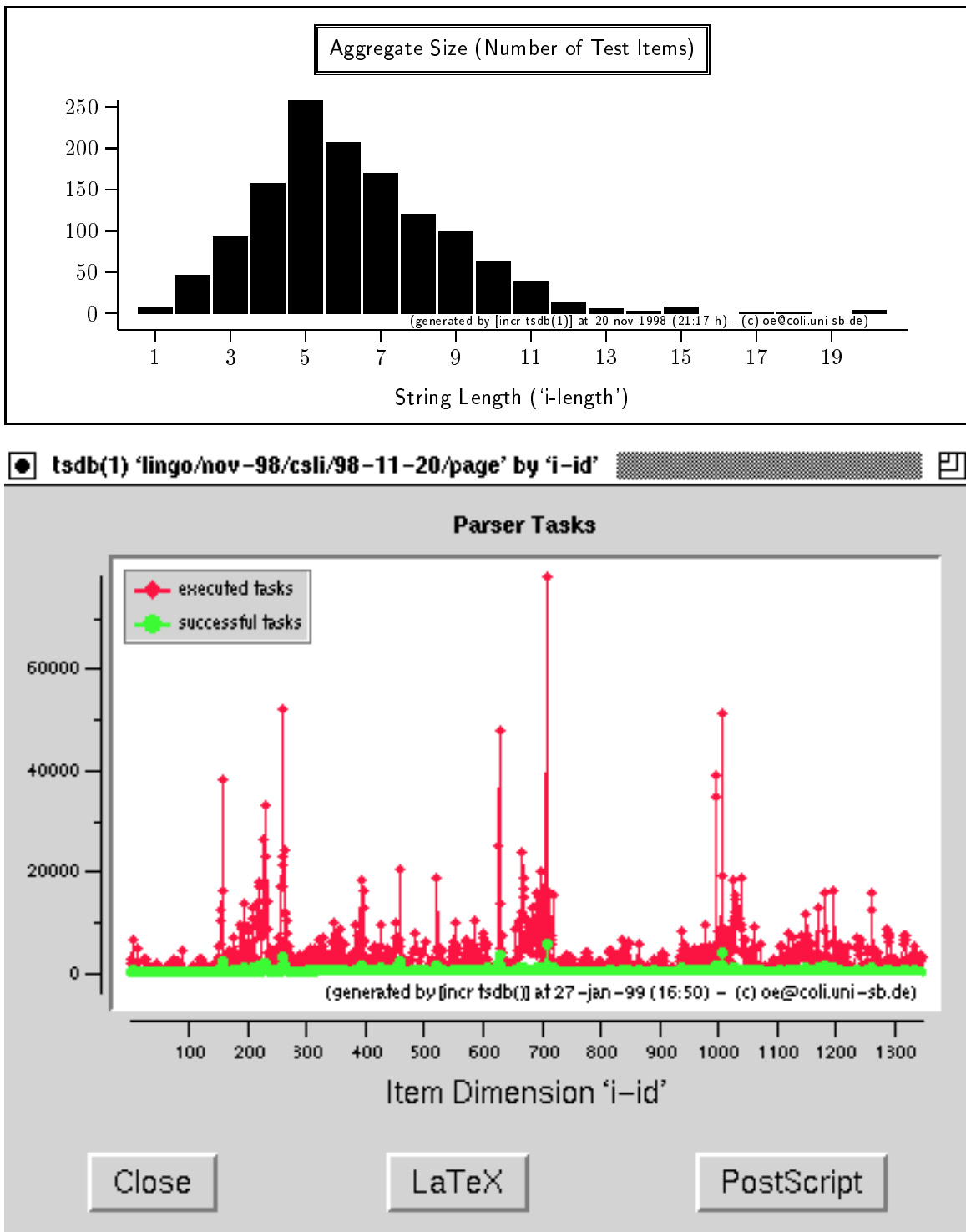
Figure 7: Barchart distribution of aggregate size by string length (top) and graphical distribution of parser tasks throughout test run (bottom); the graphs suggest that the test set is very sparsely populated with test items longer than twelve words and that parsing complexity differs immensely across the test set.
