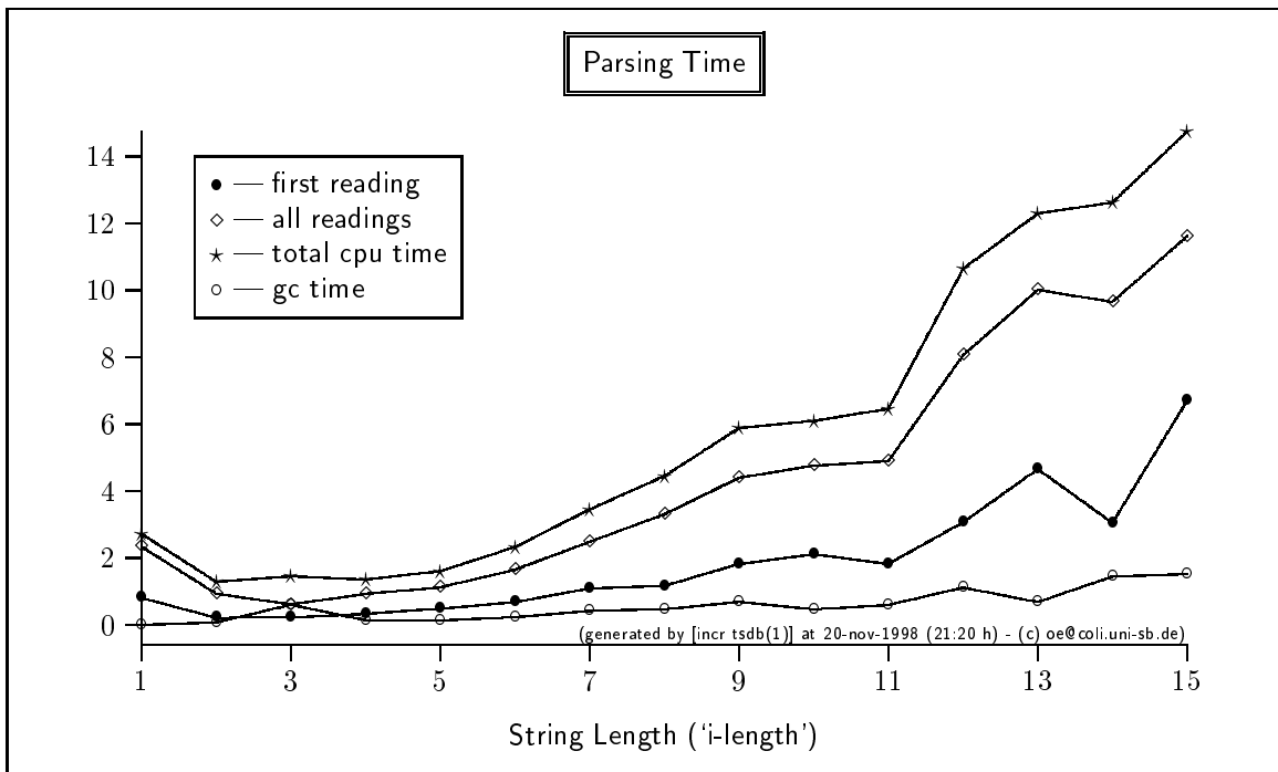
Figure 8: Graphical view of various parsing time metrics in [incr tsdb()] (encapsulated) PostScript (top) and P I CT E X (bottom) formats; both formats are fully scalable in size; as of January 1999, only the PostScript output mode allows logarithmic scaling of axes, though.
