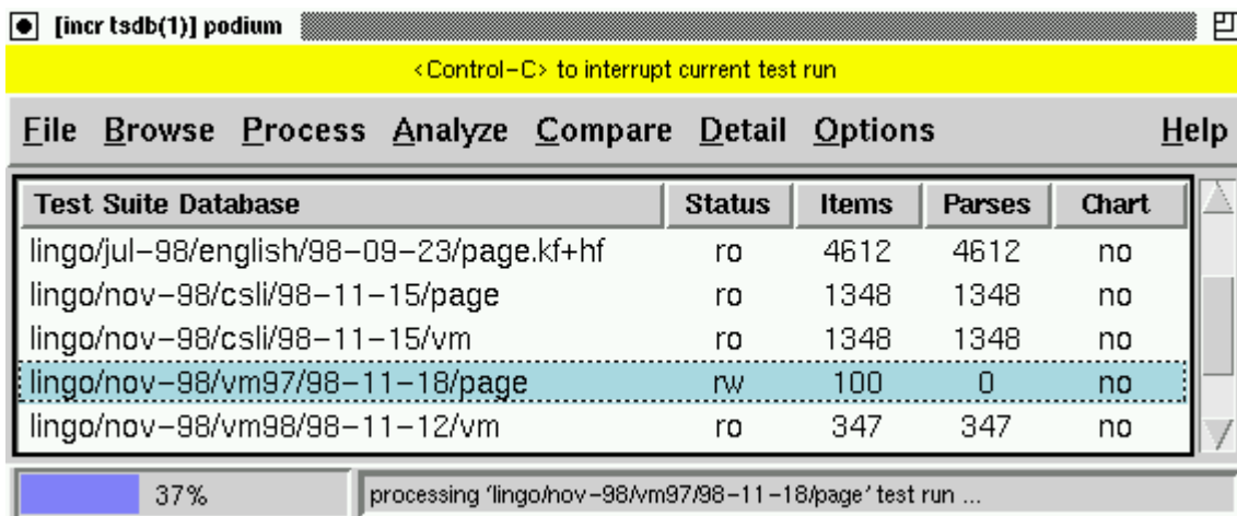
Figure 2: Screenshot of [incr tsdb()] podium : (i) the horizontal top area displays context-dependent (balloon-type) help; (ii) the menu structure reflects the prototypical profiling sequence: browsing the available data, processing and analysis of individual profiles, and comparison and in-detail study among profiles; (iii) the podium body lists all currently available profiles and their key properties; (iv) the progress meter gives an estimate of the remaining work to complete the current task; finally, (v) the lower left minibuffer serves for status messages and parameter input; when idle, the progress meter displays a digital clock.
